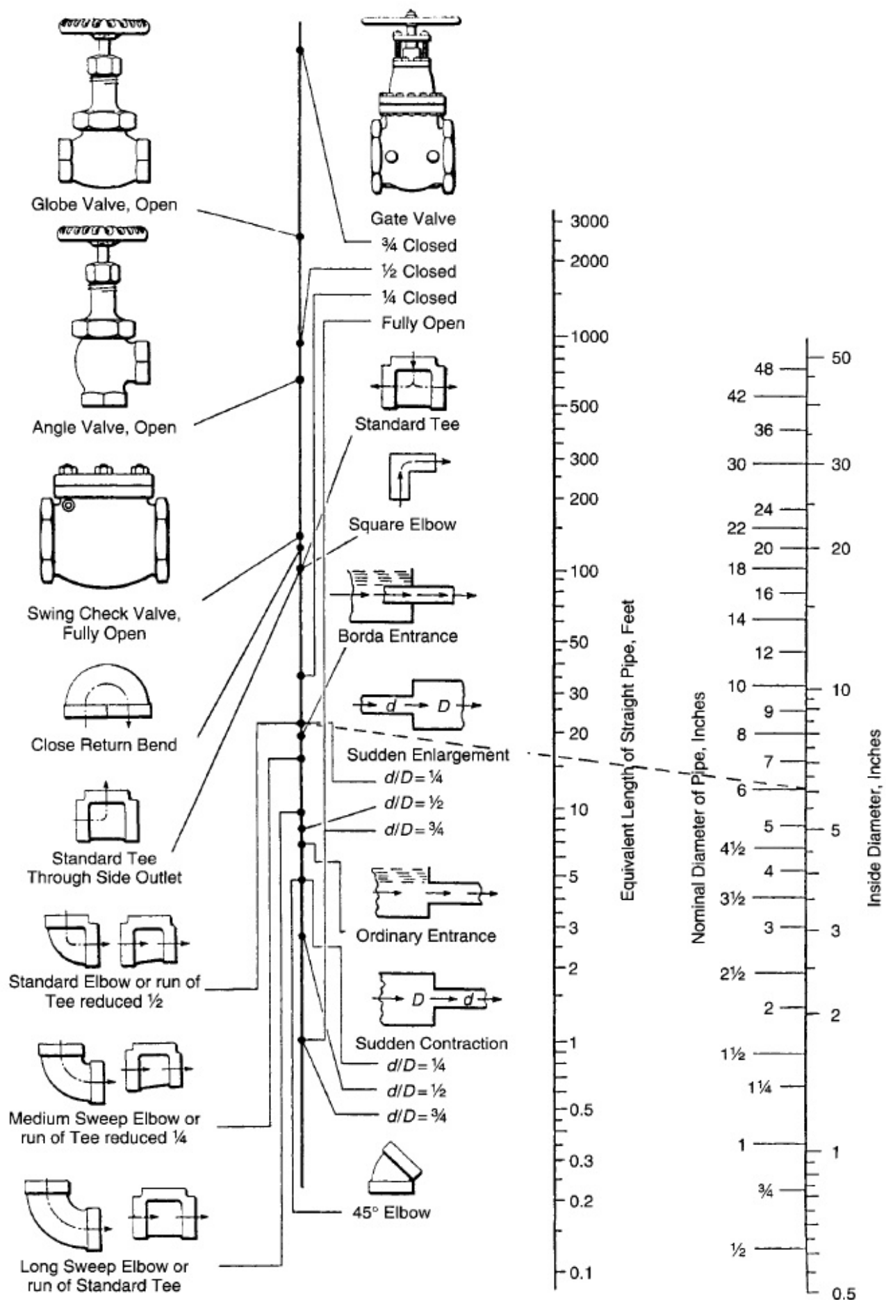
Figure 4-24a Equivalent length resistance of valves and fittings to flow of fluids. Note: Apply to 2 in. and similar threaded pipe for process applications
